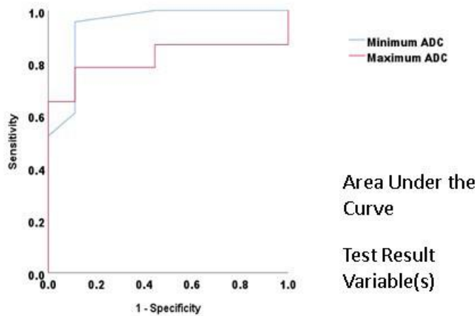
Figure 4: Test Results variability of Minimum and Maximum ADC
